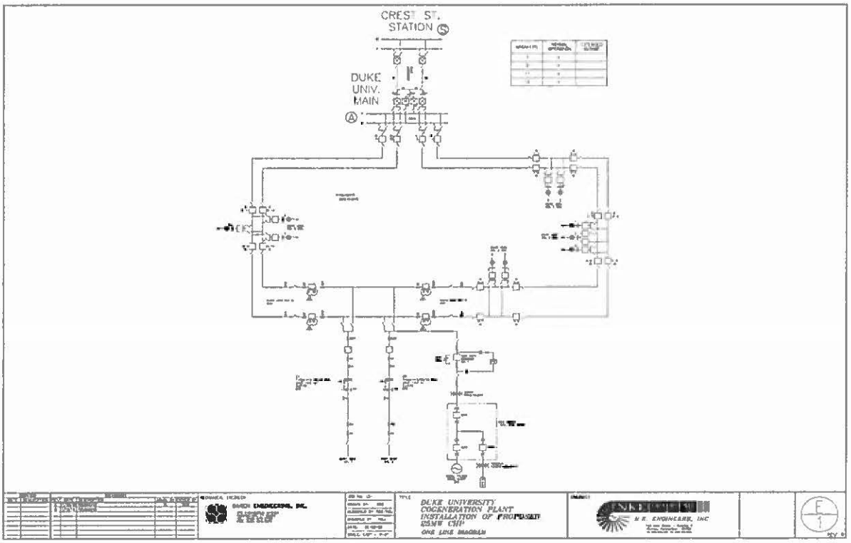
Figure 4: Single-Line Drawing
