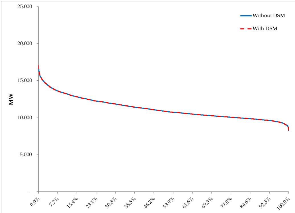
2028 Load Duration Curve
