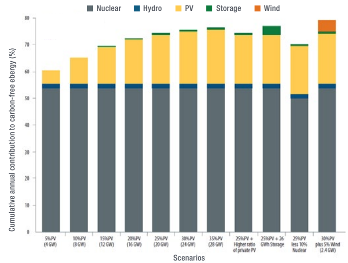
FIGURE 6 // Cumulative annual contribution to carbon-free energy (Duke Energy/NREL) 76
