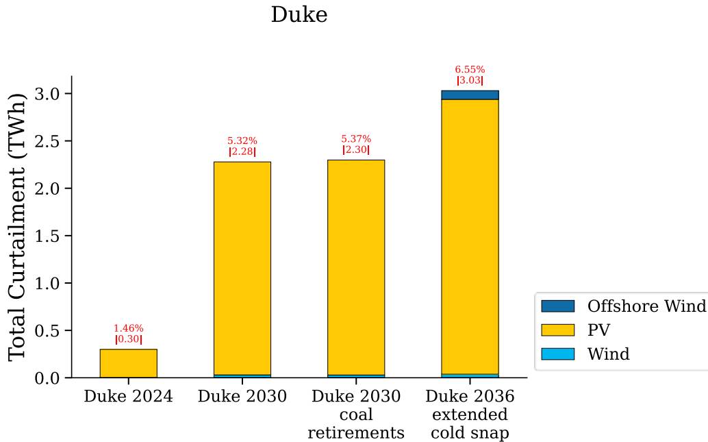
Figure 48. VRE total curtailment for the 2024 base case and 2030 case
