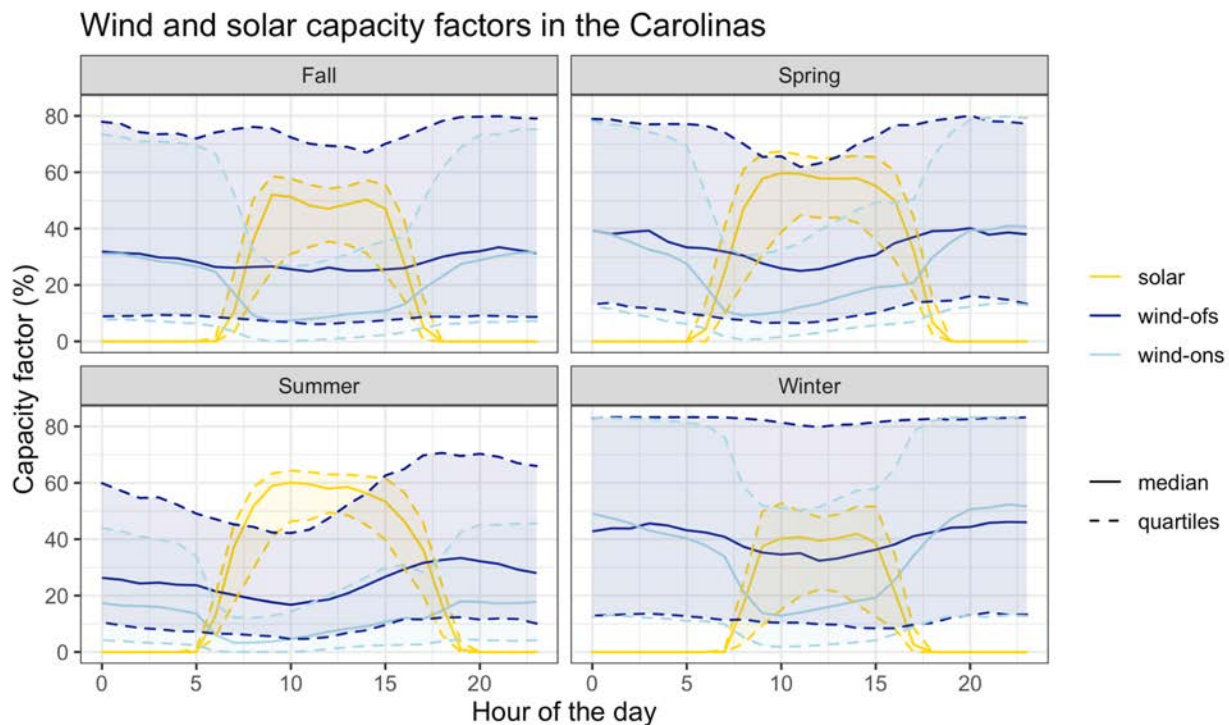
Figure 22. Solar PV, offshore wind, and land-based wind profiles for the Carolinas by season
