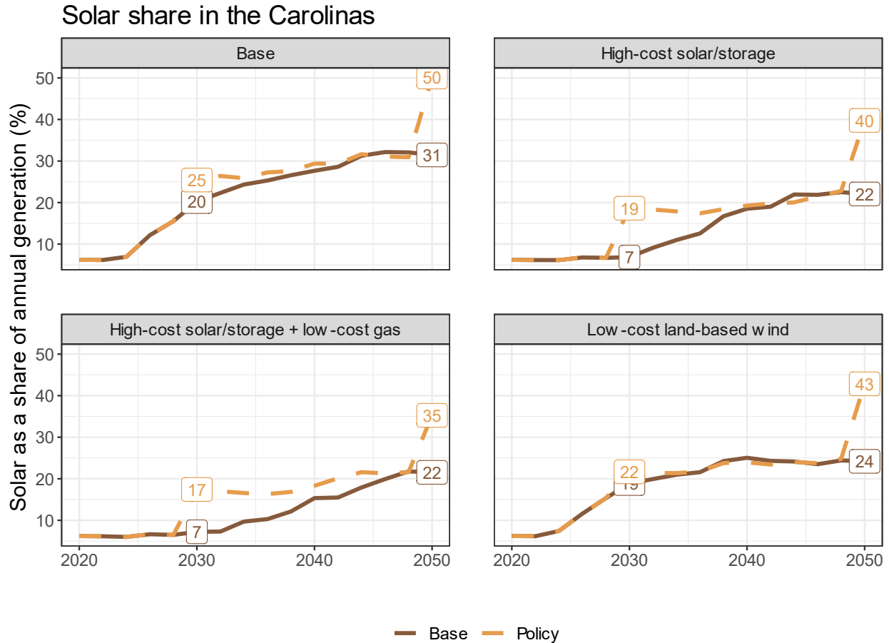
Figure 34. Annual generation from solar PV in the Carolinas (percentage of total generation) for the cost sensitivities
