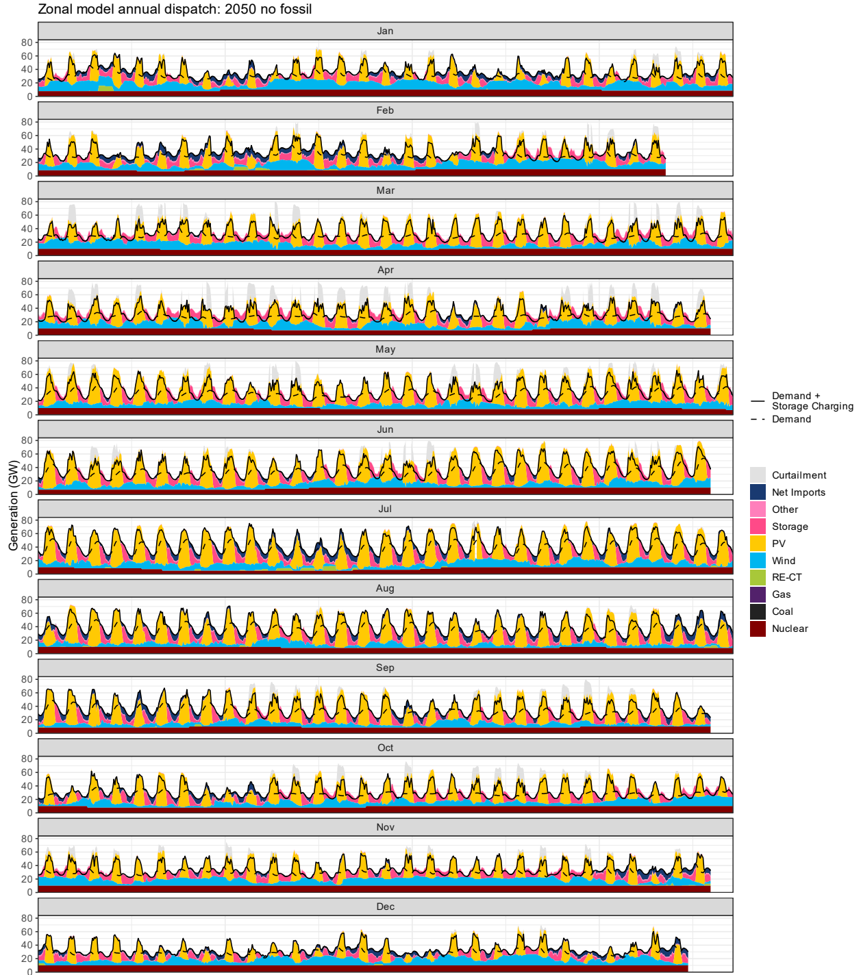
Figure B-7. Annual hourly generation by fuel type in the zonal model for the Carolinas 2050 policy no-fossil scenario
