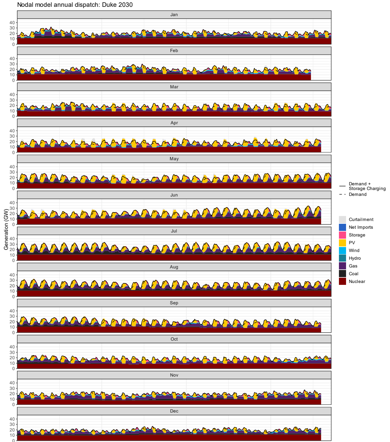
Figure B-2. Annual hourly generation by fuel type in the nodal model for the Duke 2030 scenario
