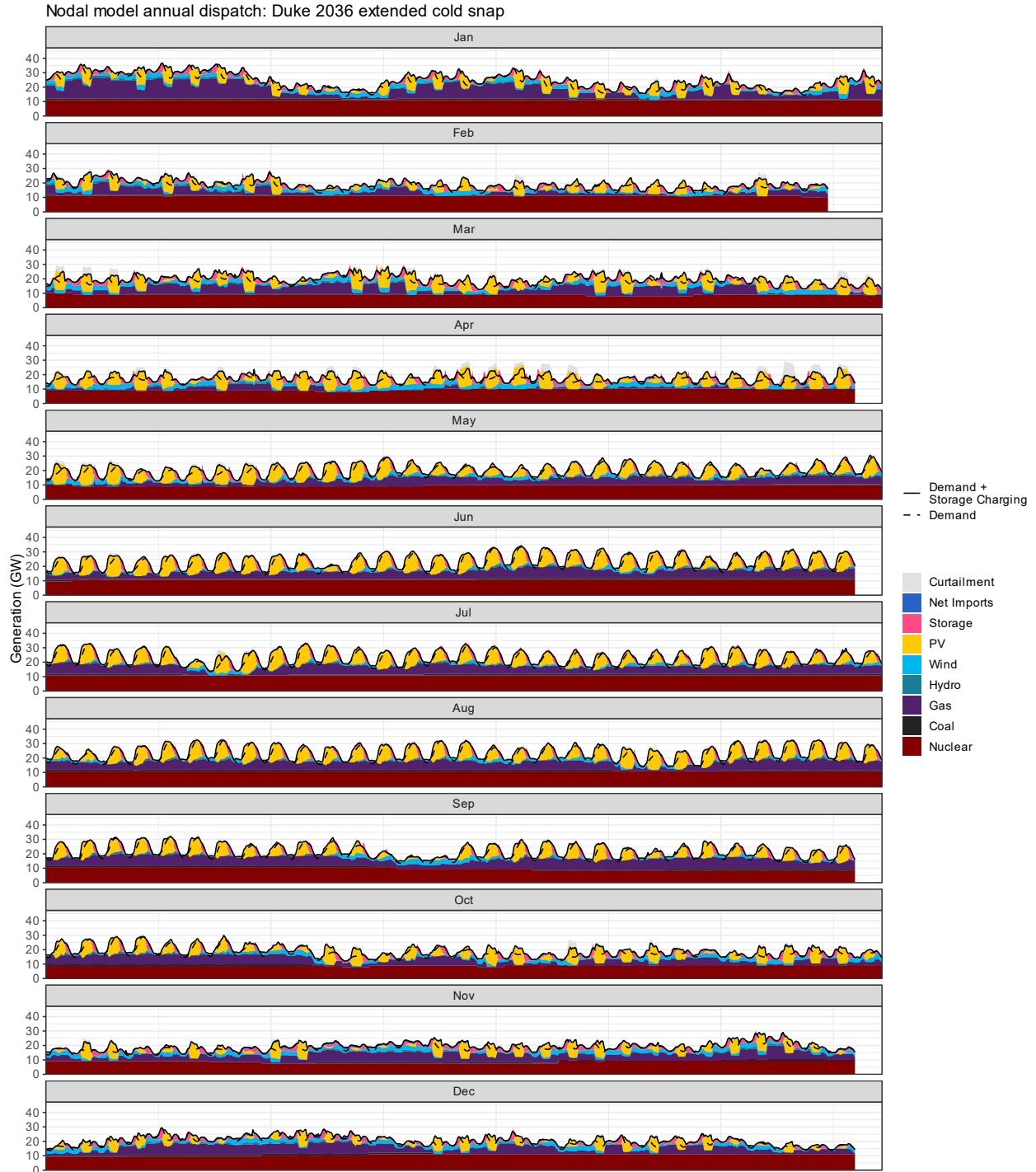
Figure B-4. Annual hourly generation by fuel type in the nodal model for the Duke 2036 extended cold snap scenario
