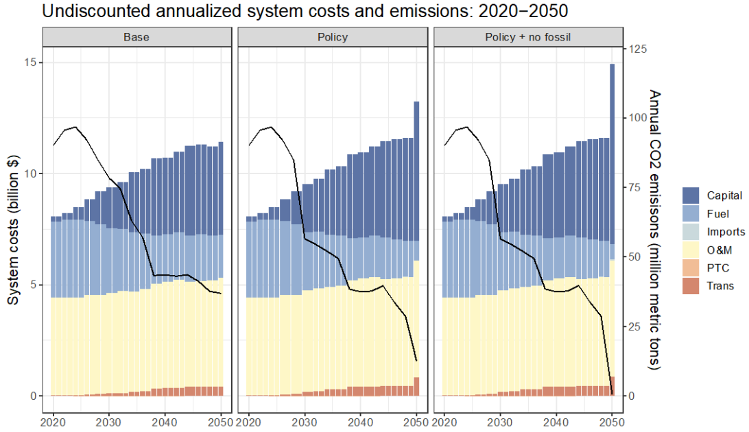
Figure 29. Annualized undiscounted system costs for the Carolinas by scenario for 2020–2050 (2018 $U.S.)
