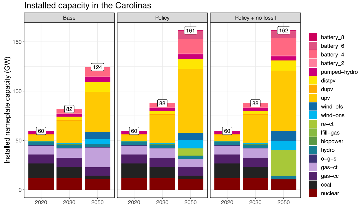
Figure 19. Installed capacity results by technology for the Carolinas for the main cases (base, policy, and policy with requirement for no fossil in 2050)
