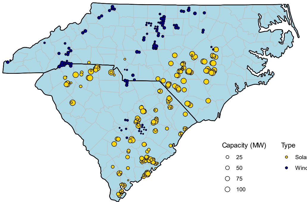
Figure 16. Map showing the placement of new utility-scale solar PV and wind resources to build the 2030 nodal PLEXOS model
