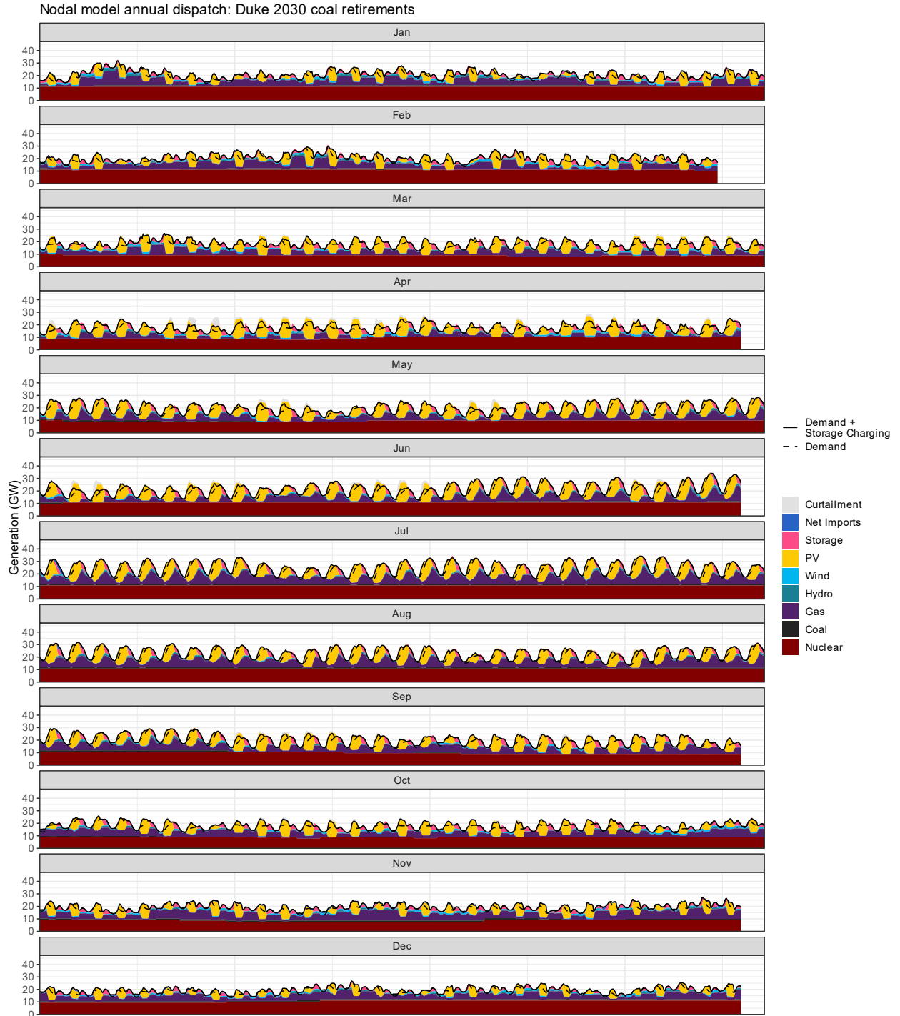
Figure B-3. Annual hourly generation by fuel type in the nodal model for the Duke 2030 coal retirements scenario
