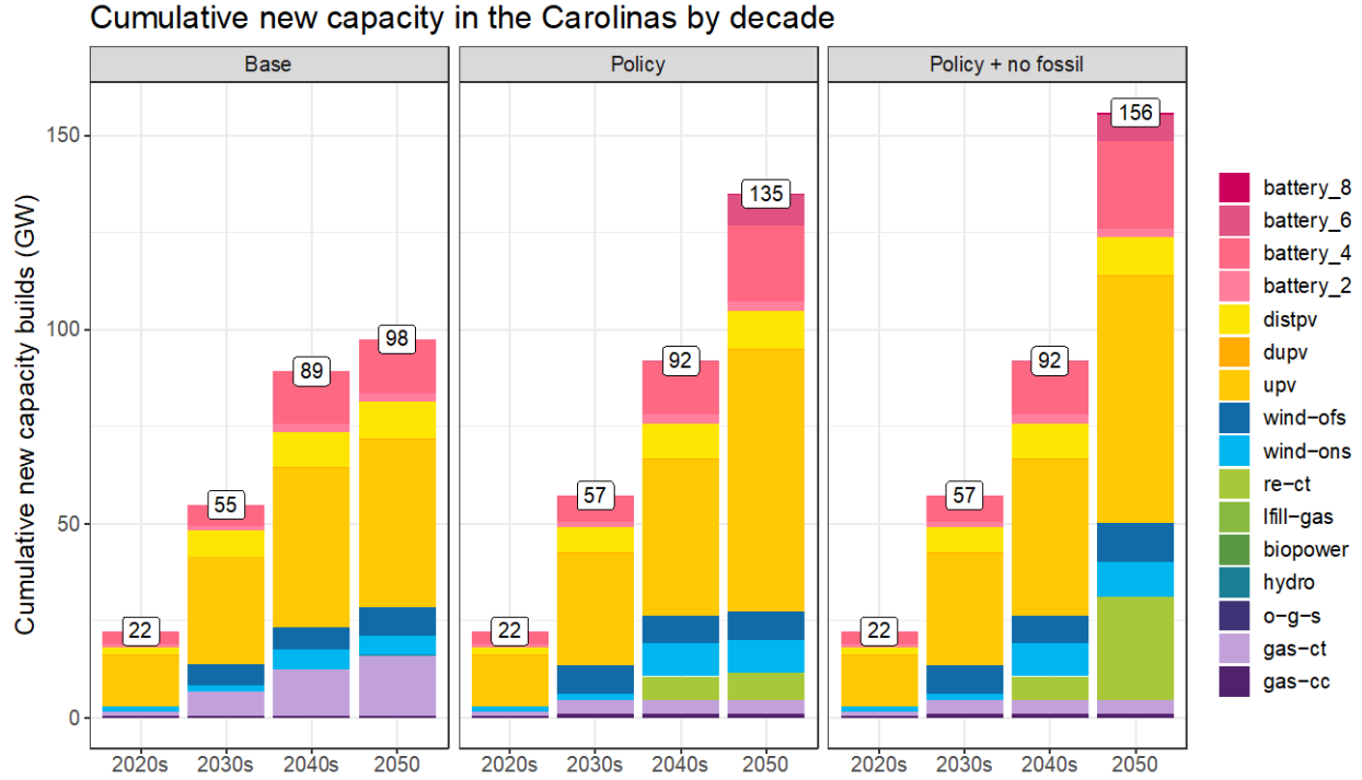
Figure 20. Cumulative new capacity builds by decade for the Carolinas
