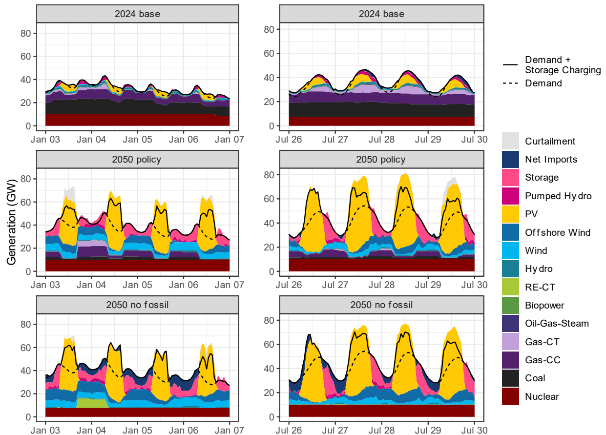
Figure 57. Generation dispatch for the 4 days surrounding the hour of net load peak in the winter (left) and summer (right)
