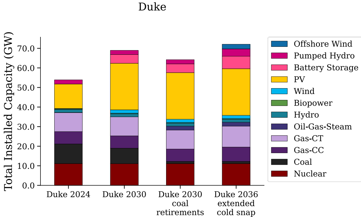
Figure 42. Total installed generation capacity in Duke Energy’s territory in each case used in the nodal production cost modeling
