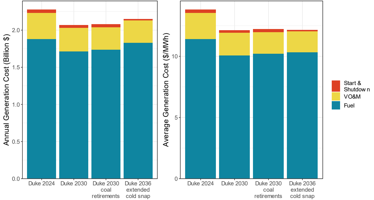
Figure 51. Annual generation costs for the nodal production cost modeling cases broken out by cost type
