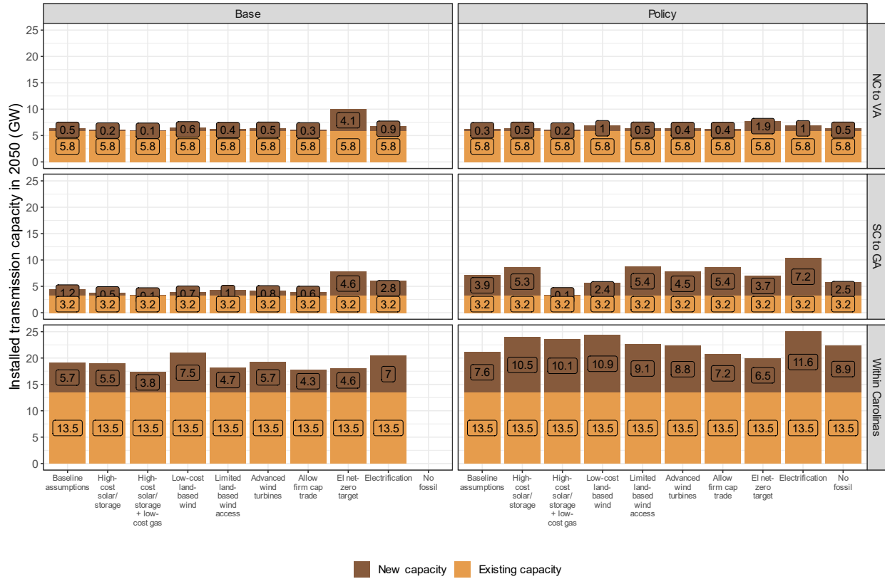
Figure 41. Installed transmission capacity (GW) in 2050 for various sensitivities in the base case and policy emissions scenarios
