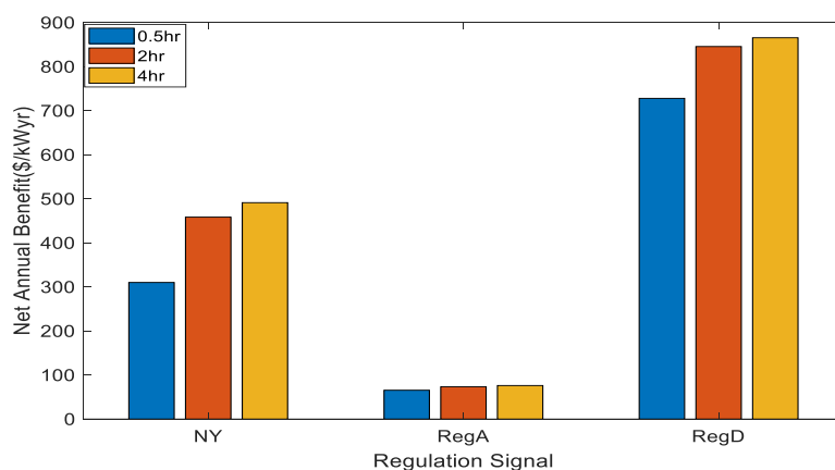
Figure 6.6.13. Comparison of net annual benefits for different Li-ion battery durations.
