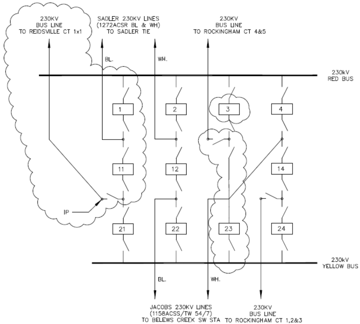
ERNEST SWITCHING STATION FUTURE CONFIGURATION
