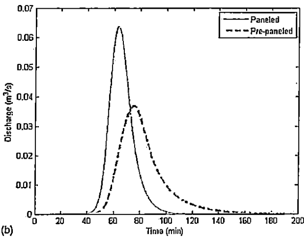
Fig. 4. Hydrograph with time increment of (a) 12 s; (b) 3 s with Manning's n for bare ground
