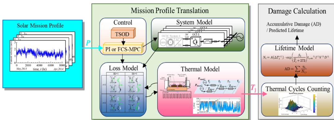
Fig. 5 Reliability assessment framework for utility PV system
