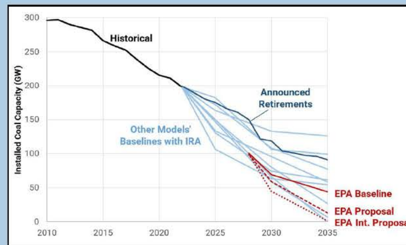
Figure B: BPS Coal-Fired Generation Capacity in Various Scenario Models—United States Only
