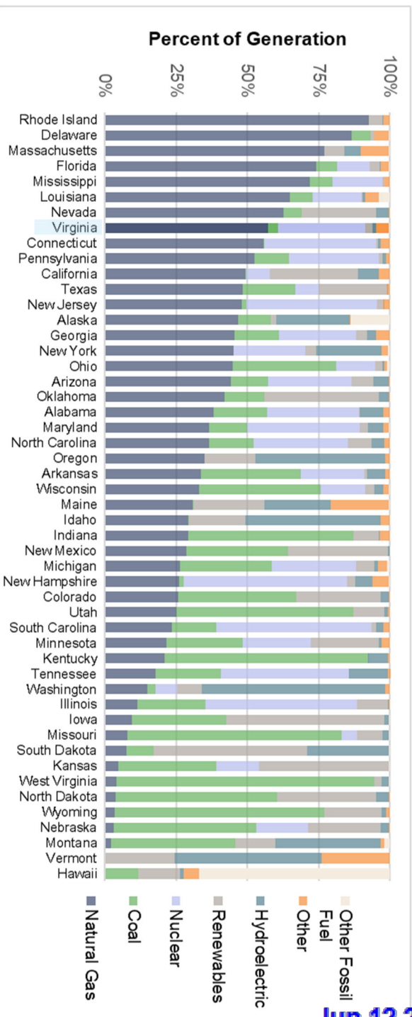
Figure 1. Electricity generation mix, as fraction of total. 1
